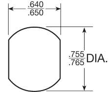
MOUNTING CUTOUT
